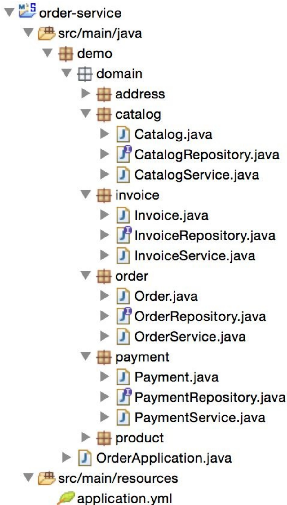
Figure 9-4. Package structure for the Order context
