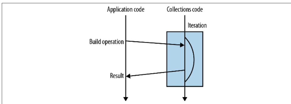
Figure 3-2. Internal iteration
